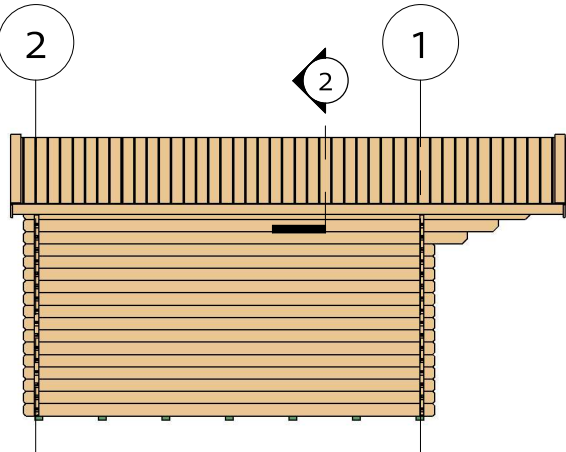
Roof 2
