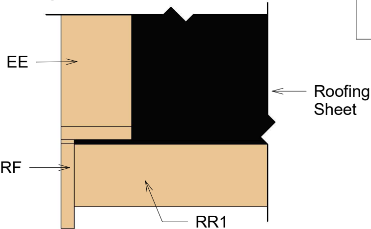
③ Roof Reinforcement
